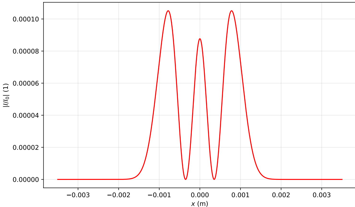
Intensity profile I(x, y = 0, z = 0.239)/I_0 , P_{in}=3.0P_{cr} , artificial time
